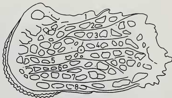
Fig. 8 Hermanites percultus sp. nov. Paratype OS 8227. Carapace from left, lateral surface showing the ornament. \times 110 . 1–8, the ridges described in the text.
